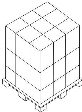
The pallet stack drawing
